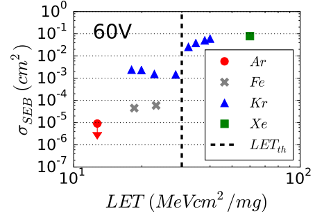
Fig. 11: Heavy ion SEB data as a function of LET for the power MOSFET biased at 60V. All values were obtained with at least 50 events except for Ar, for which no events were observed and corresponds to the two-sigma upper limit.
