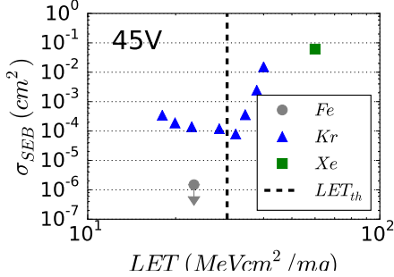
Fig. 10: Heavy ion SEB data as a function of LET for the power MOSFET biased at 45V. All values were obtained with at least 50 events except for Fe, for which no events were observed and corresponds to the two-sigma upper limit.
