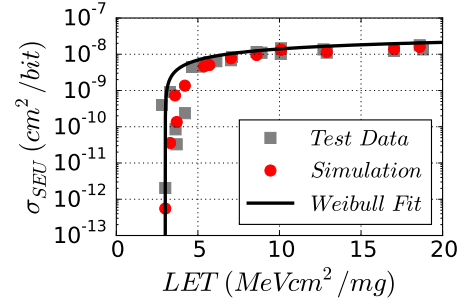
Fig. 3: Response function that optimizes the fit of the simulated values to the test data.
