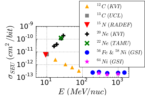
Fig. 2: Sub-threshold heavy ion test data as a function of energy per nucleon.
