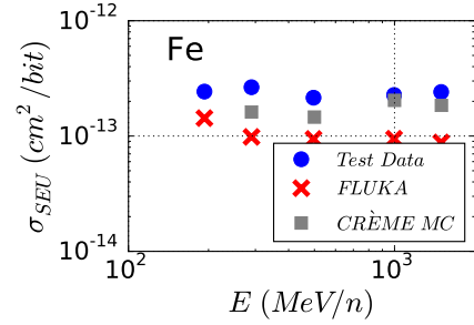
Fig. 6: Simulated SEU cross sections for Fe ions as a function of ion energy compared to experimental results.
