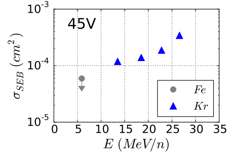
Fig. 12: Heavy ion SEB data in the sub-LET threshold region as a function of energy for the power MOSFET biased at 45V. All values were obtained with at least 50 events except for Fe, for which no events were observed and corresponds to the two-sigma upper limit.
