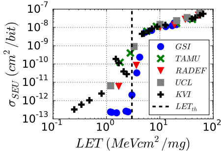
Fig. 1: Heavy ion test data as a function of LET.
