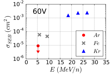
Fig. 13: Heavy ion SEB data in the sub-LET threshold region as a function of energy for the power MOSFET biased at 60V. All values were obtained with at least 50 events except for Ar, for which no events were observed and corresponds to the two-sigma upper limit.
